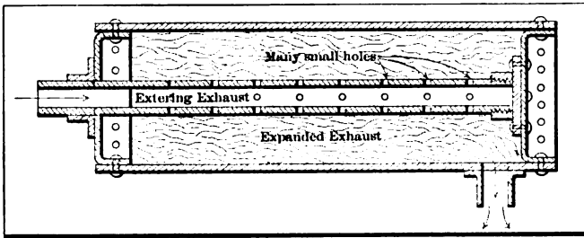
Fig. 62—Depicting a simple form of muffer, used on many cars, and delivering good satisfaction
